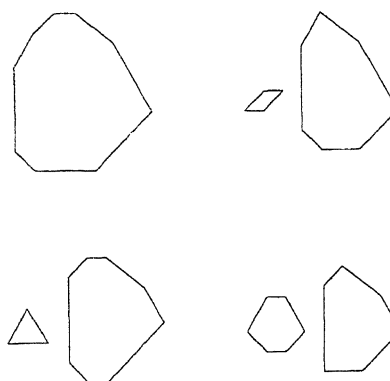
Fig. 7. From left to right and top to bottom: the original polygon P and its decomposition with respect to rotation over 180^\circ , rotation over 120^\circ , and reflection in the vertical axis.
